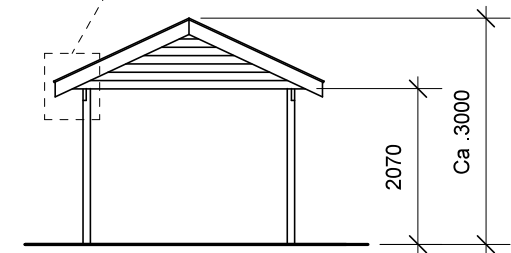
Front gavl
