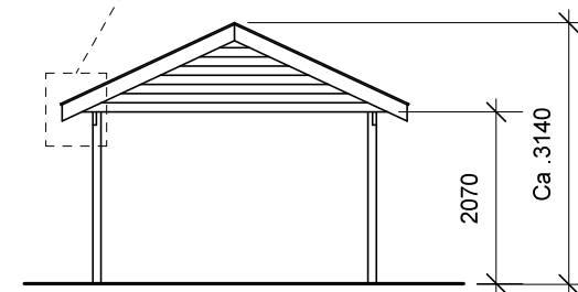
Front gavl
