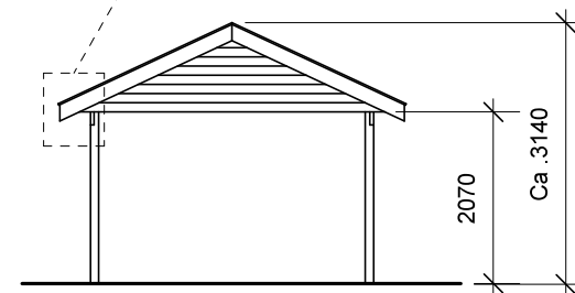
Front gavl
