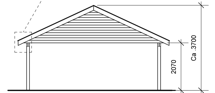
Front gavl
