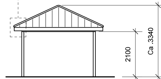
Front gavl
