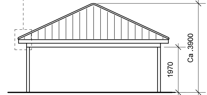
Front gavl
