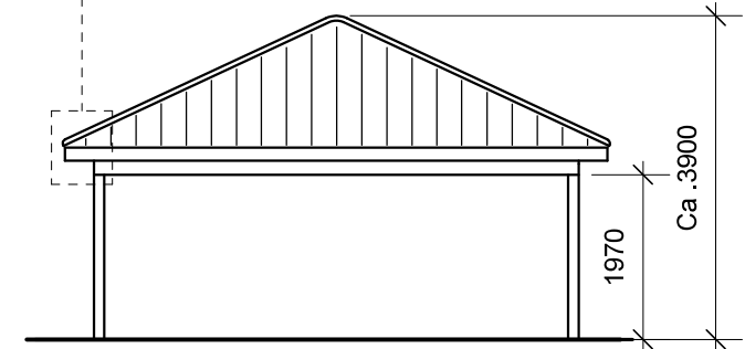
Front gavl
